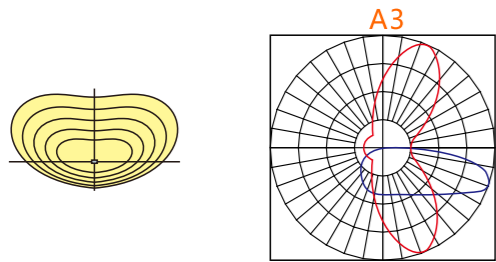
Distribution: A3 Applicable to two-way, 6-lanes or wider roadway, tunnel and area lightings.
