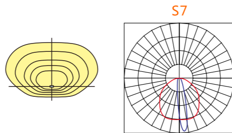
Distribution: S7 Applicable to wall washing, for instance architecture, park and community lightings.
