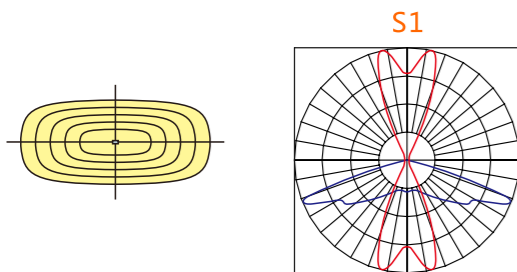
Distribution: S1 Applicable to roadway, tunnel, factory and venue lightings;
