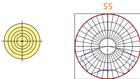
Distribution: S5 Applicable to projection, high-mast, architecture, stadium and factory lightings.
