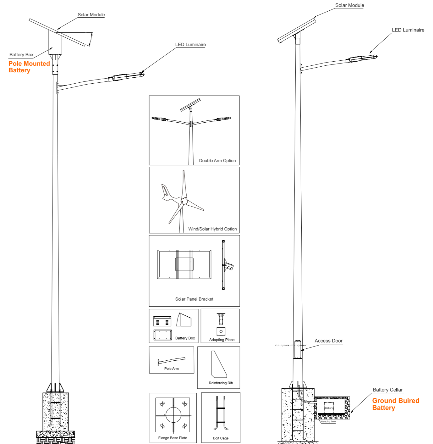
Pole Height:6M/8M
