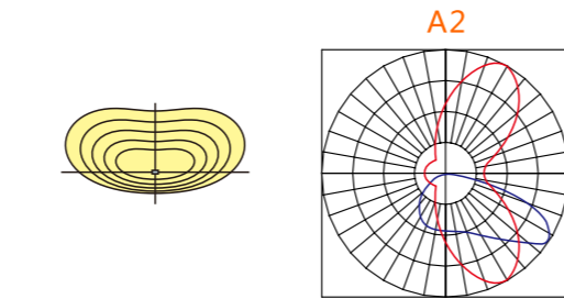
Distribution: A2 Applicable to two-way, 6-lanes or narrower roadway, tunnel and area lightings.
