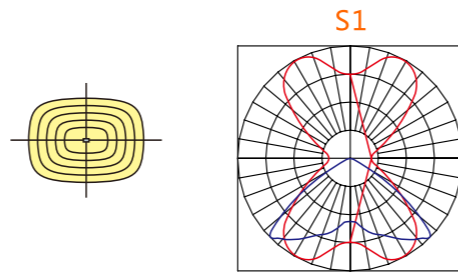
Distribution: S1 Applicable to roadway, tunnel, factory and venue lightings;
