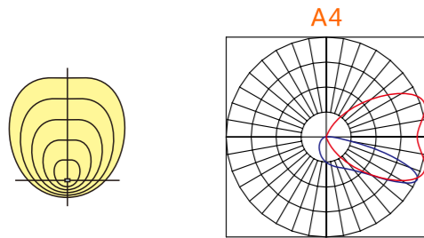
Distribution: A4 Applicable to intersection, parking-lot, area lightings, and high-mast, billboard and low space lightings.
