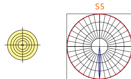
Distribution: S5 Applicable to projection, high-mast, architecture, stadium and factory lightings.
